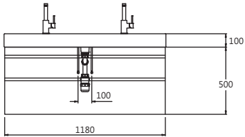
EH05348D/DW/DW1/DTG
